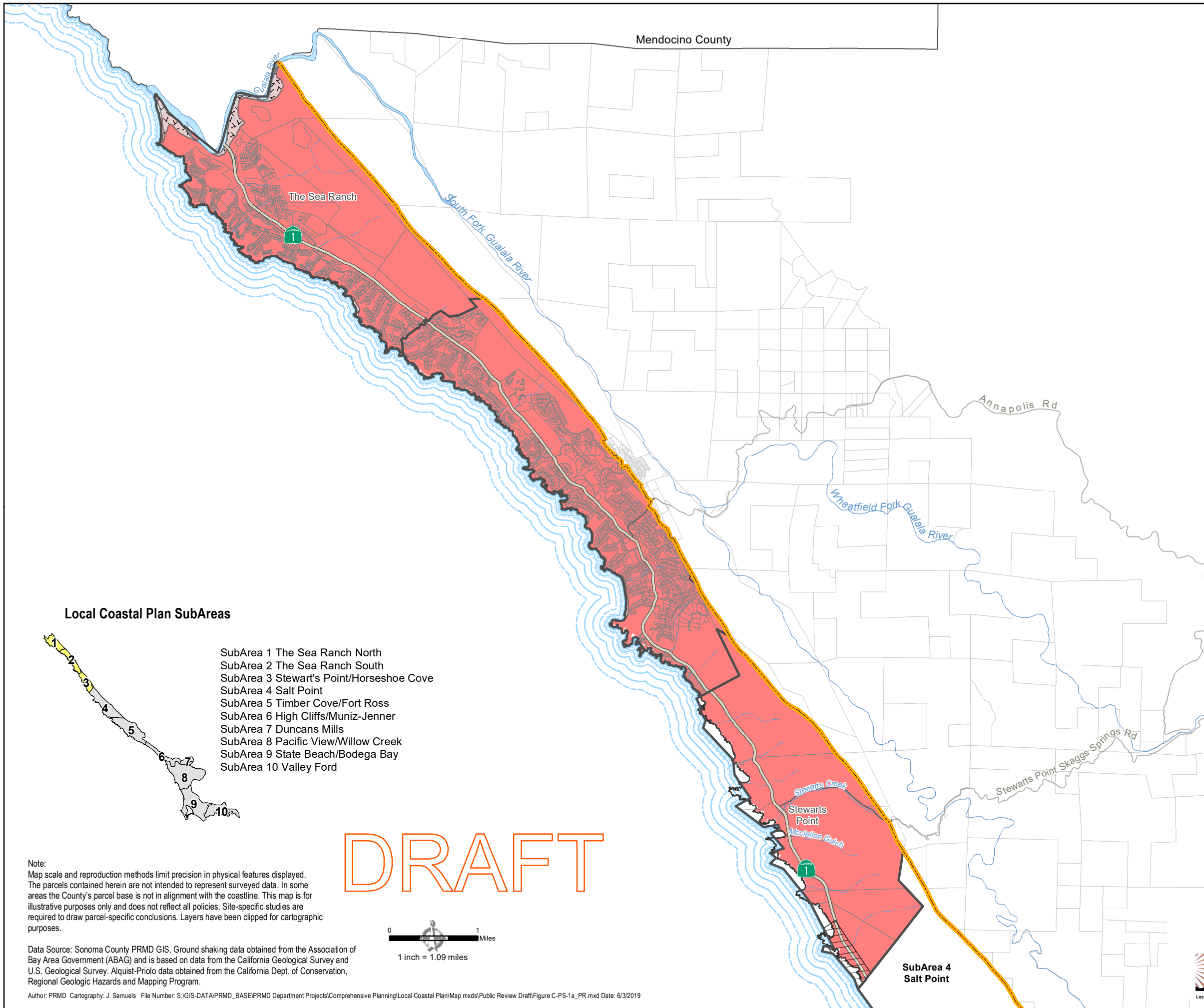
FIGURE C-PS-1a Seismic Geologic Hazards SubAreas 1 - 3
