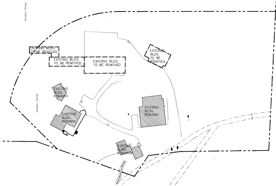
EXISTING BUILDINGS ① 1"=40'-0"
